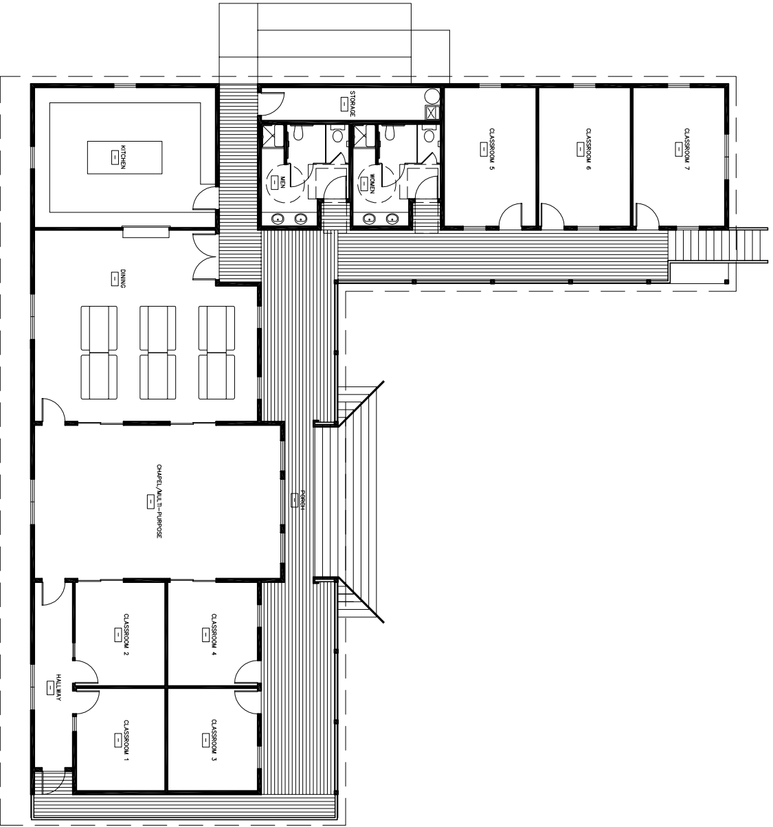
PRELIMINARY FLOOR PLAN - OPTION 1
